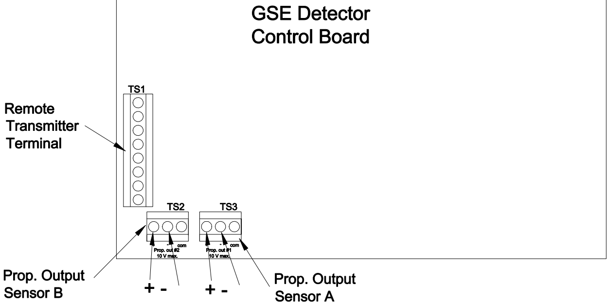
Fig. 7: Location of GSE proportional output terminals.
